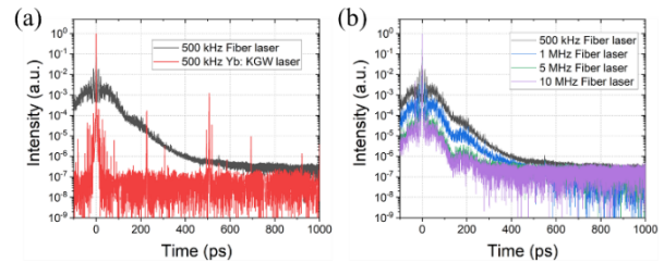
Fig. 4. Temporal contrast ratio of 300 fs pulses from Yb:KGW and fiber lasers over a time range of -100 to 1000 ps. (a) Comparison of the contrast ratio at a repetition rate of 500 kHz for both lasers. (b) Contrast ratio for fiber laser at various repetition rates.
